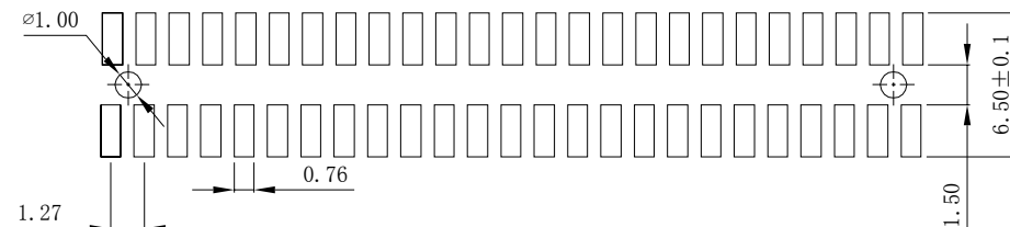
PCB Layout
